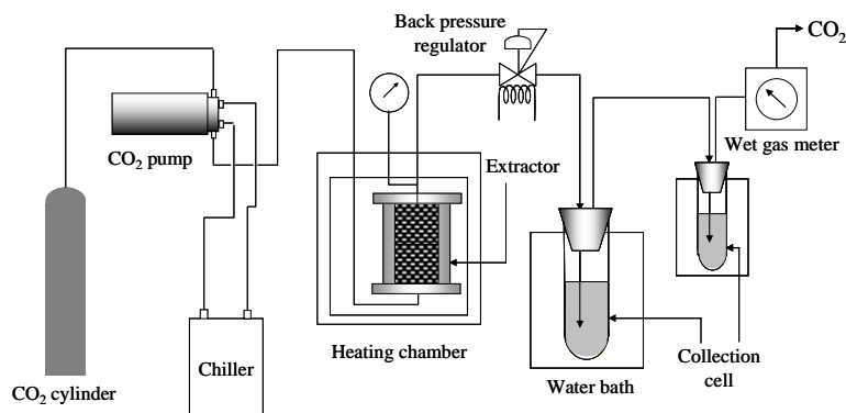
Figure 1. Schematic diagram of supercritical CO 2 apparatus
