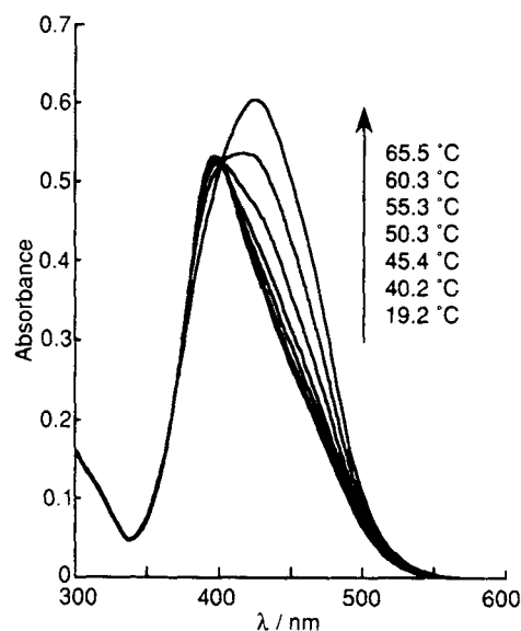
Fig. 1 Temperature dependence of visible spectra of 2 in the presence of 1 in benzene. [\mathbf{1}] = 2.0 mmol l -1 , [\mathbf{2}] = 2.0 mmol l -1 . Path length of cell; 0.1 mm.
